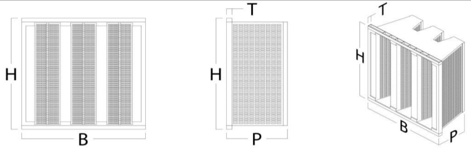
Reference drawing: vefim_ftrvr
